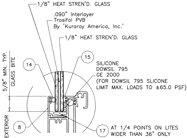
GLAZING DETAIL 5/16" OVERALL LAM. GLASS
