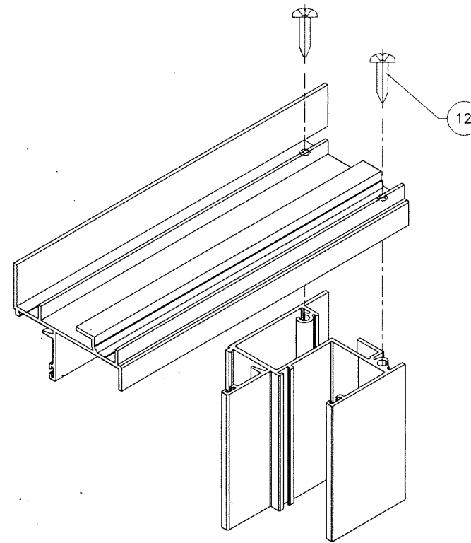
FRAME TOP CORNER
